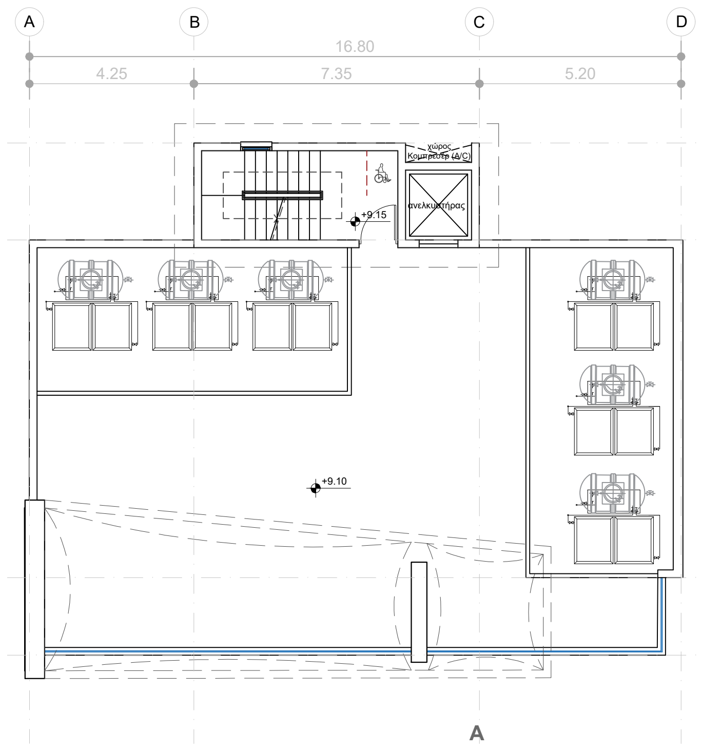
BLOCK A - Roof Plan
