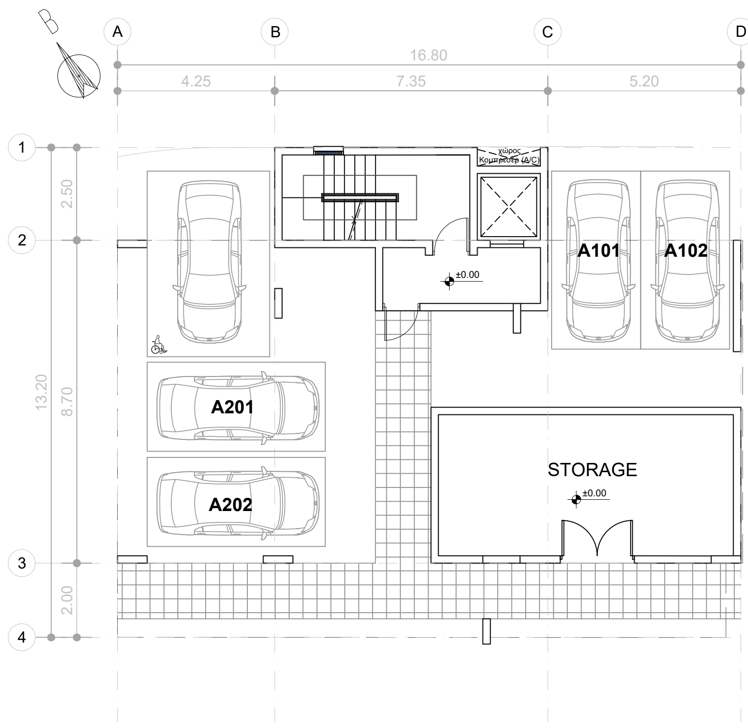
BLOCK A - Ground Floor
