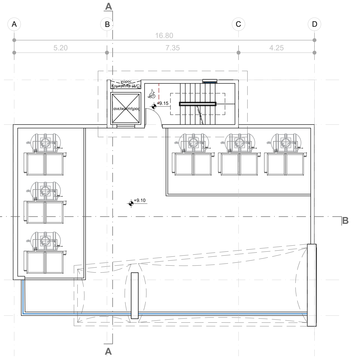
BLOCK C - Roof Plan
