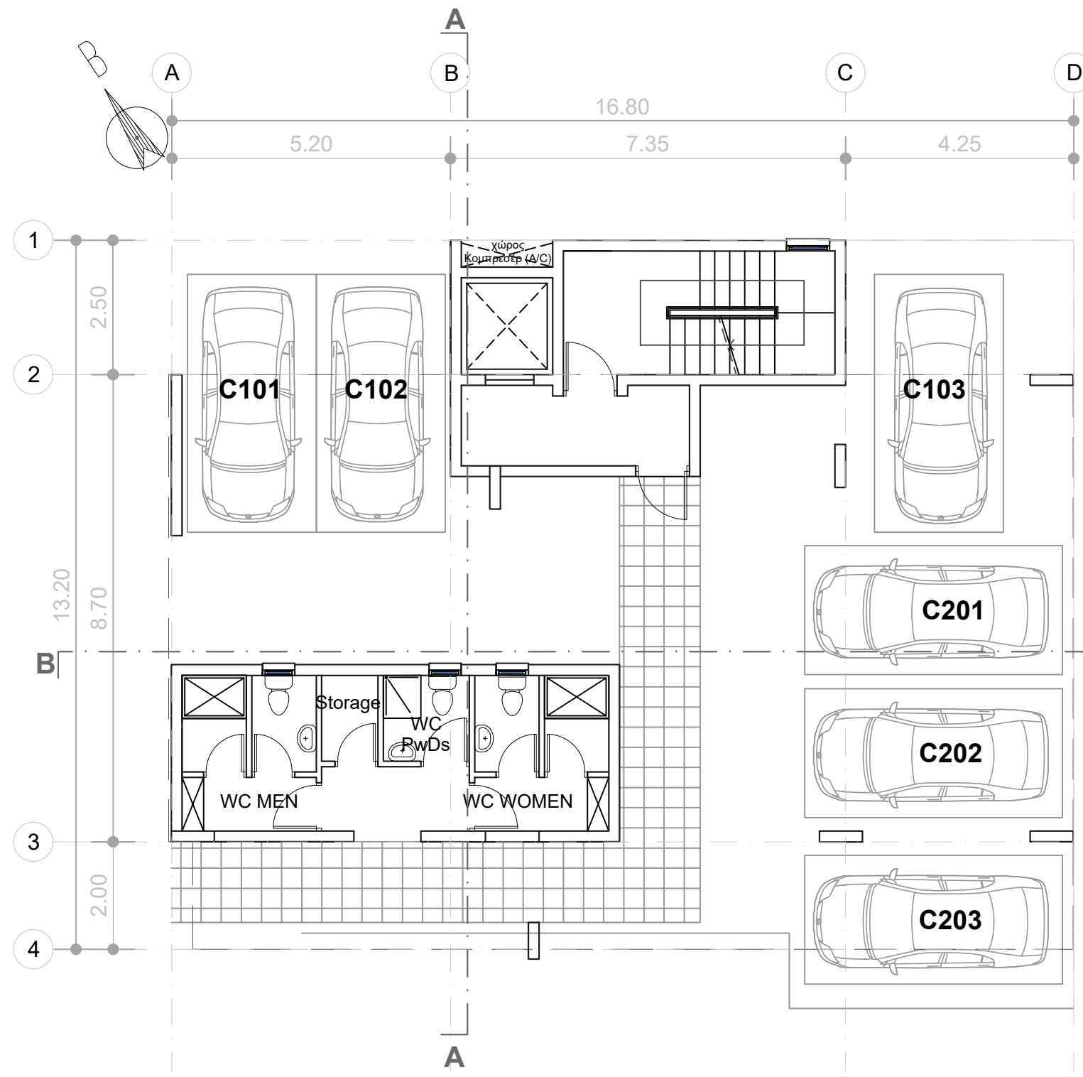
BLOCK C - Ground Floor
