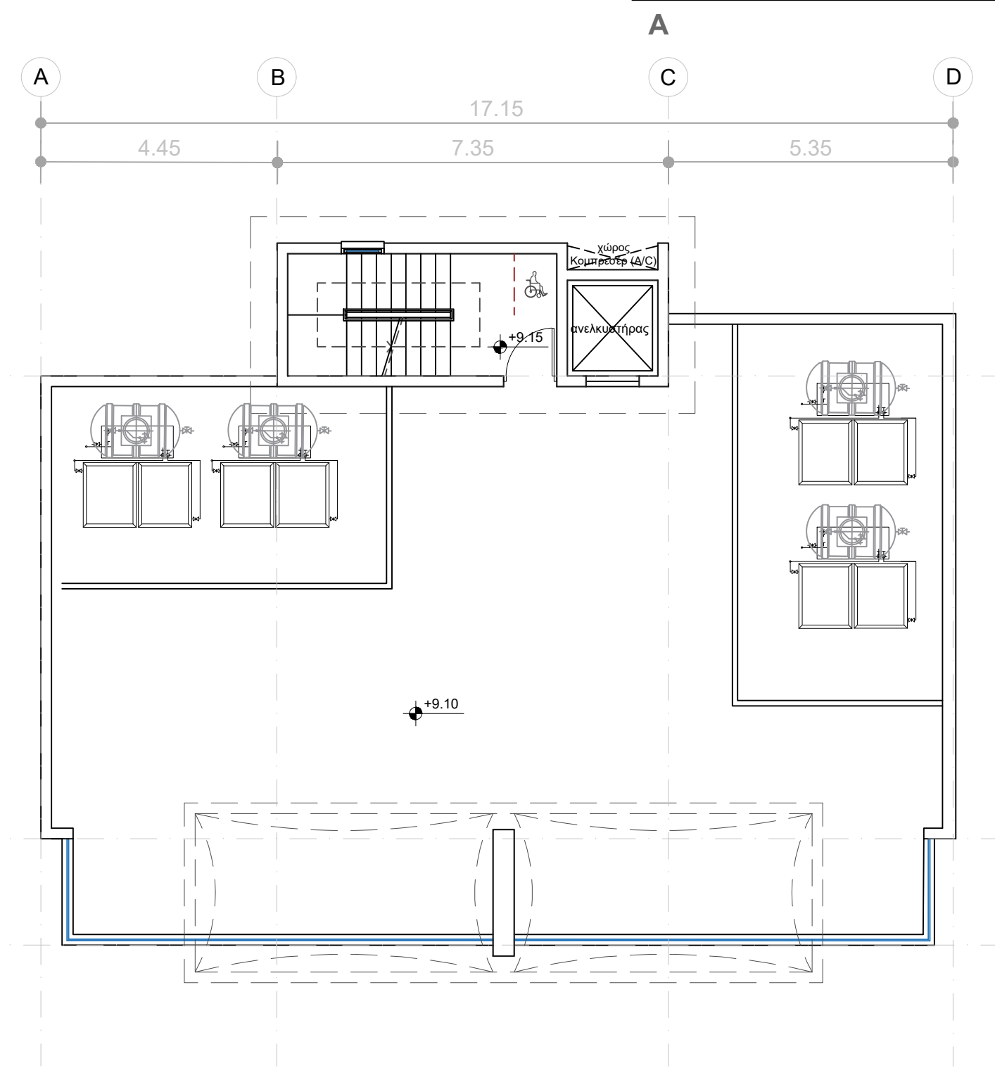
BLOCK B - Roof Plan
