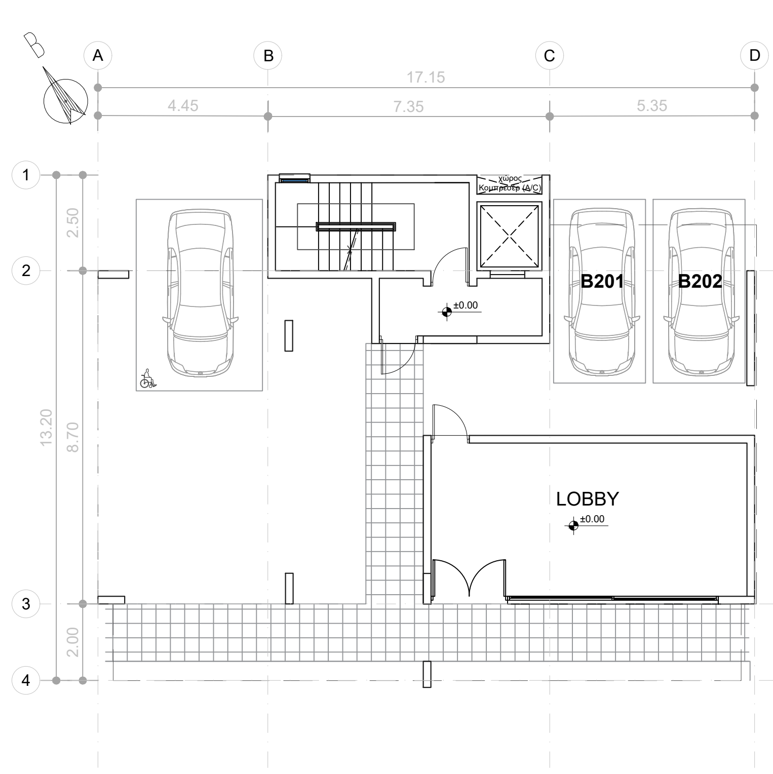
BLOCK B - Ground Floor
