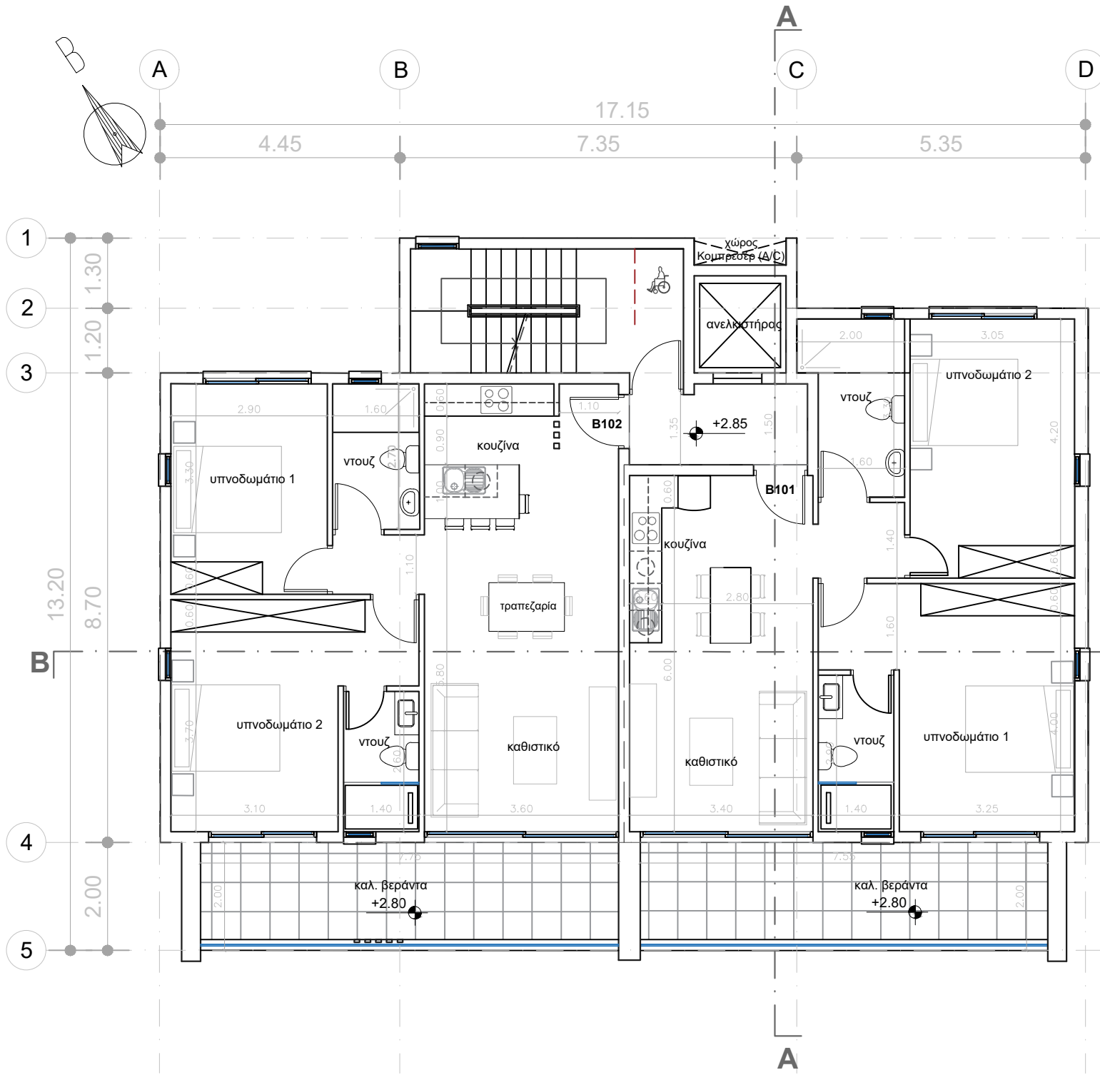
BLOCK B - First Floor
