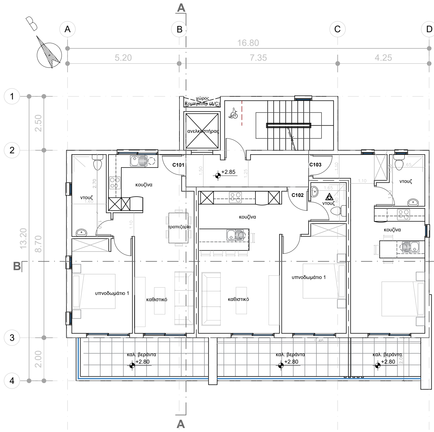
BLOCK C - First Floor
