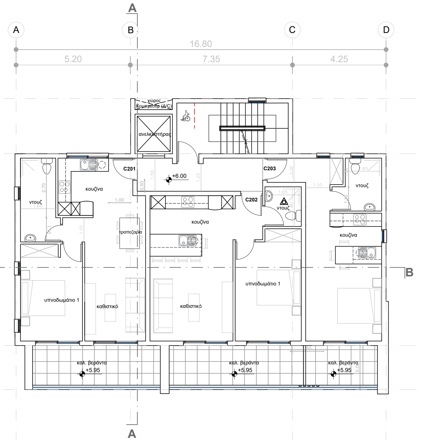
BLOCK C - Second Floor
